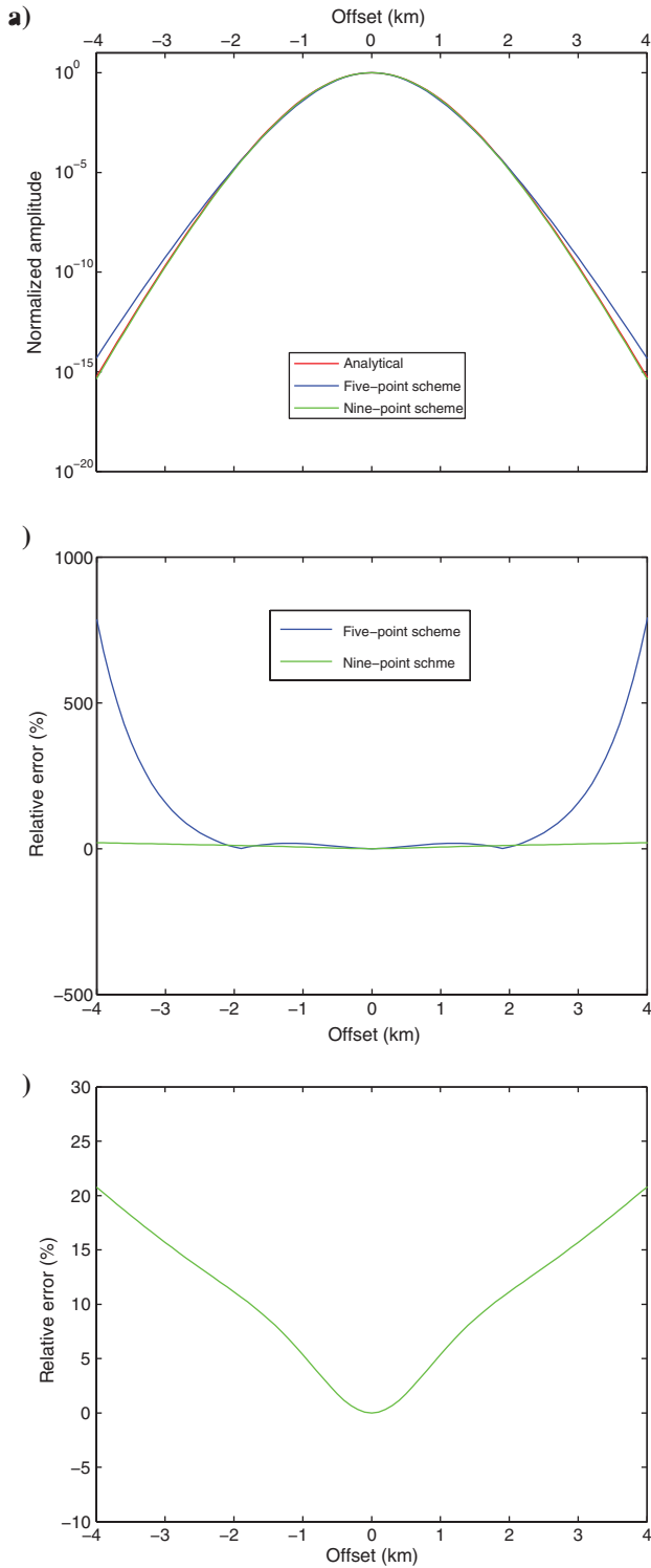
Figure 4. Laplace-domain seismograms computed with the analytical formula (equation 11), the classic five-point scheme (equation 5), and the average-derivative optimal nine-point scheme (equation 2) (a), the corresponding relative errors (b), and an enlarged part of (b) in (c). The Laplace damping constant s is 10\pi , \Delta x = 100 m, and \Delta z = 50 m.
